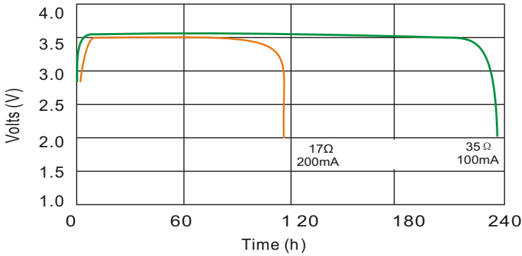
Voltage plateau versus Current and Temperature
