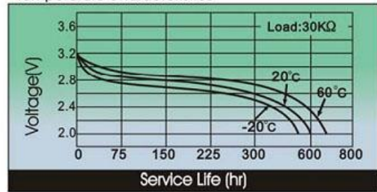
Temperature Characteristics
