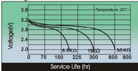
Discharge Characteristics
