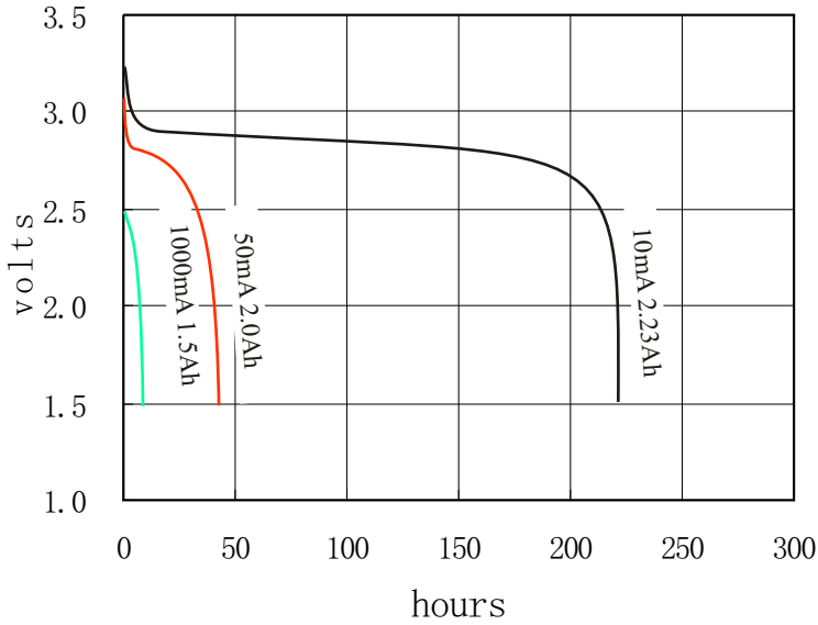
Voltage plateau versus Current and Temperature
